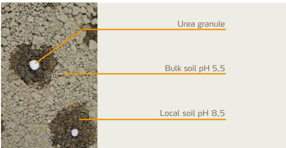
Figure 2: Hydrolysis of urea temporarily and locally increases soil pH, resulting in increased ammonia losses.
