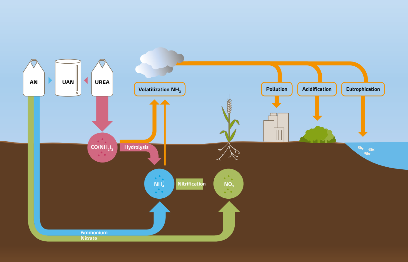
Figure 4: All mineral nitrogen fertilizer is ultimately transformed into nitrate (NO 3 - ) before it is taken up by plants. Ammonium (NH 4 + ) is an intermediate compound which is either directly applied (as ammonium nitrate NH 4 NO 3 ) or converted in the soil from urea (CO(NH 2 ) 2 ). Ammonium is in equilibrium with ammonia (NH 3 ) in the soil solution. The higher the pH, the more the balance shifts in favor of ammonia. UAN is a mix of AN and urea and thus activates all the pathways in the above diagram.
