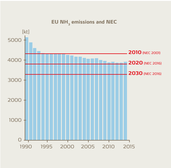
Figure 5: Ammonia emissions in the EU have decreased slowly in the past two decades. The 2016 NEC directive sets national reduction targets for 2020 and 2030, respectively.
